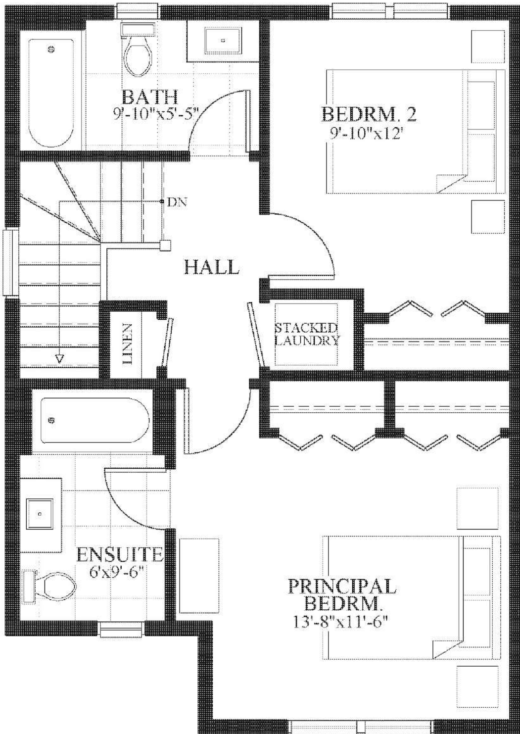
Floor Plan Level 2
