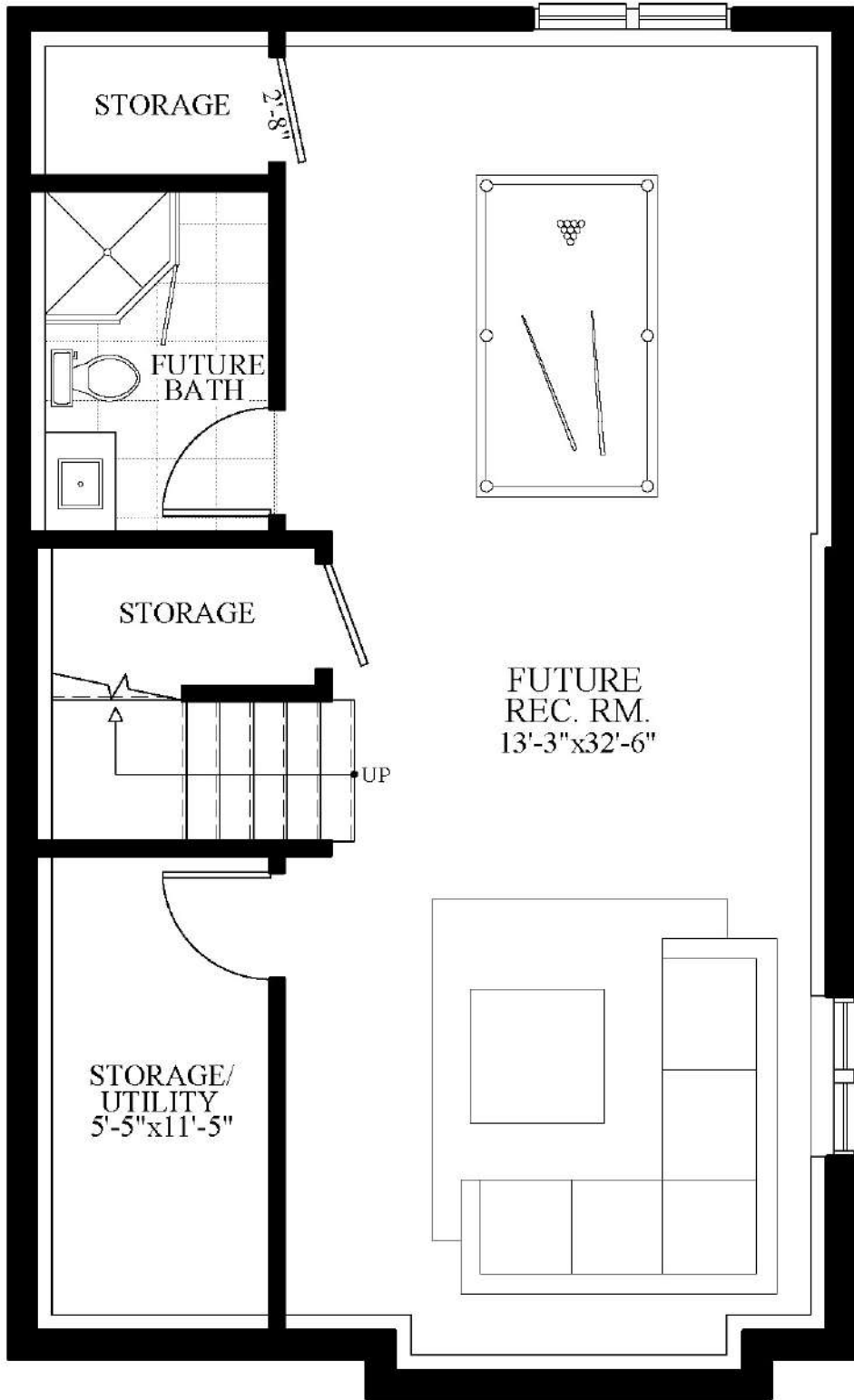
Basement Plan
