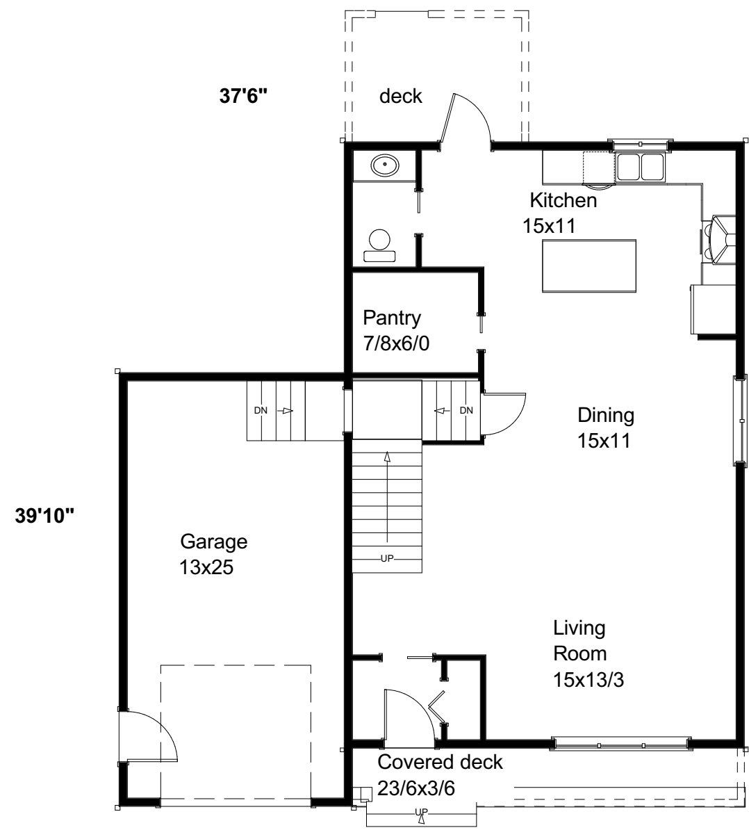
FLOOR PLAN 872SQFT
