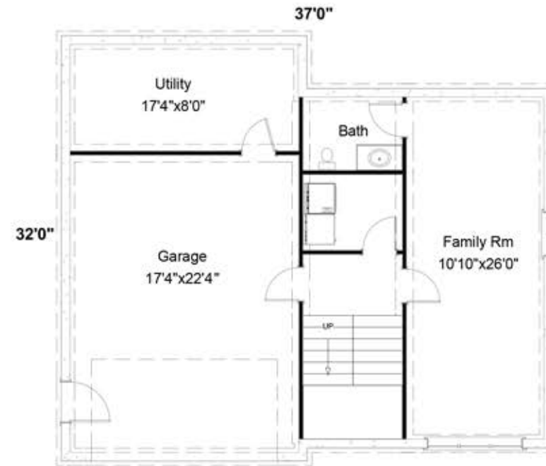
FOUNDATION PLAN
